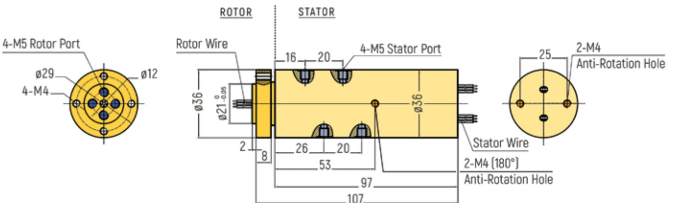
RX-PM504 - 12 Signal Rings
