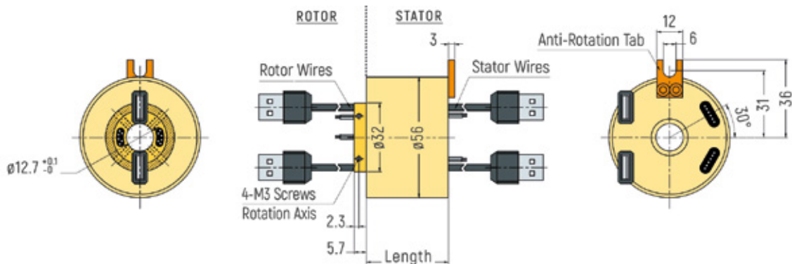
RX-USB122 - 2 USB Passages
