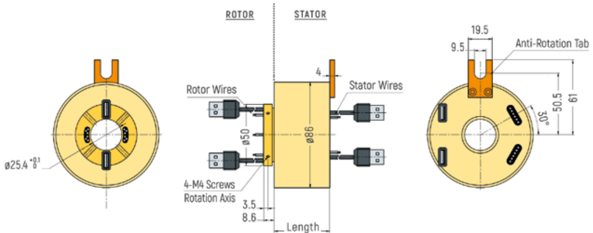
RX-USB252 - 2 USB Passages
