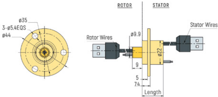
RX-USB002 - 2 USB Passages
