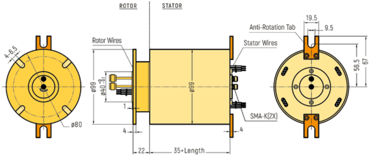
RX-HF0992 - 2 Channels
