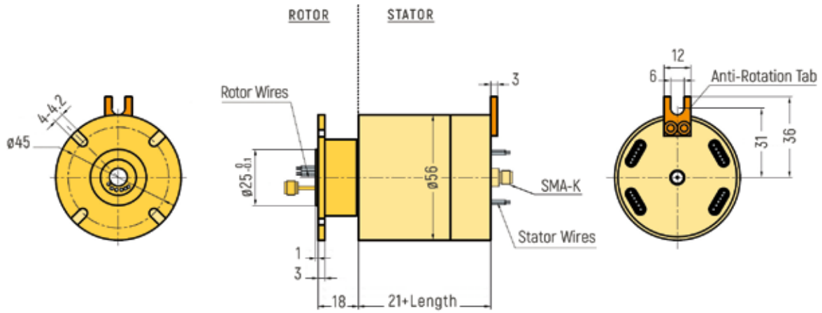
RX-HF0561 - 1 Channel
