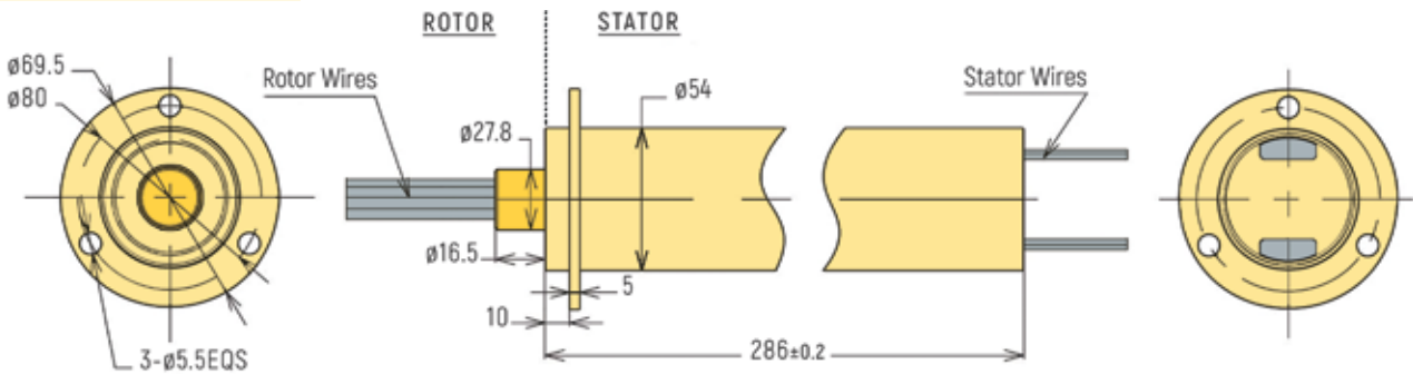
RX-MIN54A - 125 Rings / 2A
